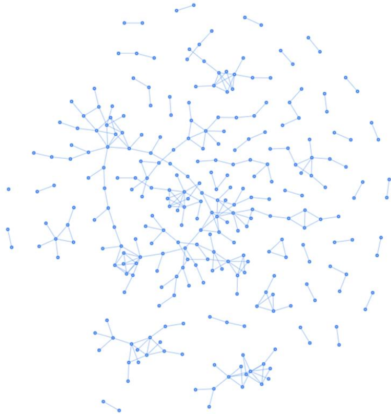
Embedding Node2Vec
