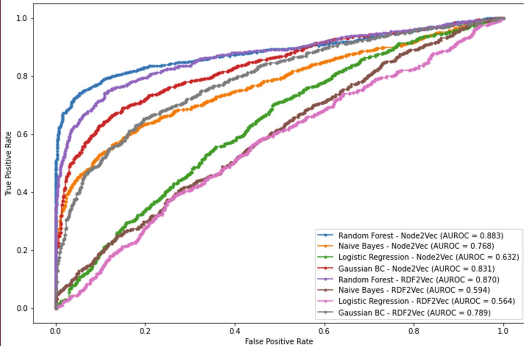
ROC Plot
